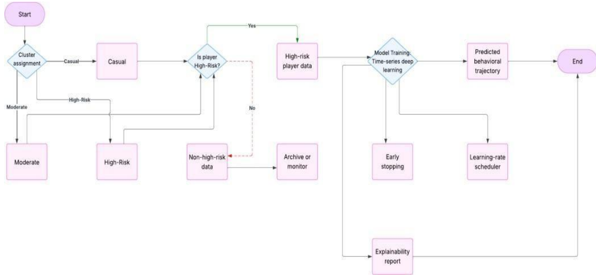
Figure 7: Workflow Diagram of Gambling Addiction Risk Prediction System
