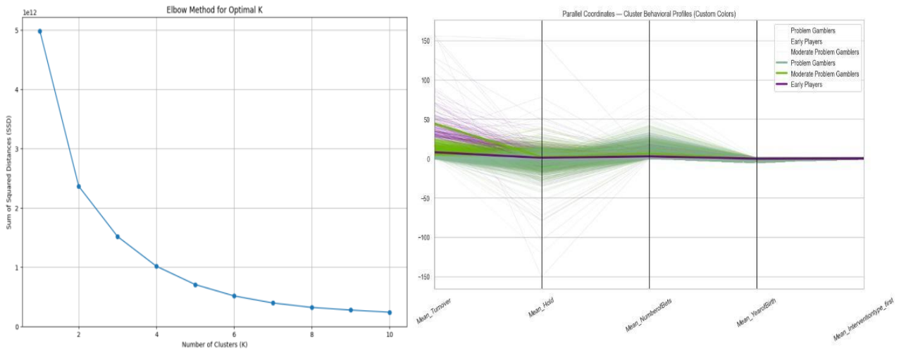
Figure 8: Elbow Method for Optimal K in left and Analysis of Cluster Labelling in right
