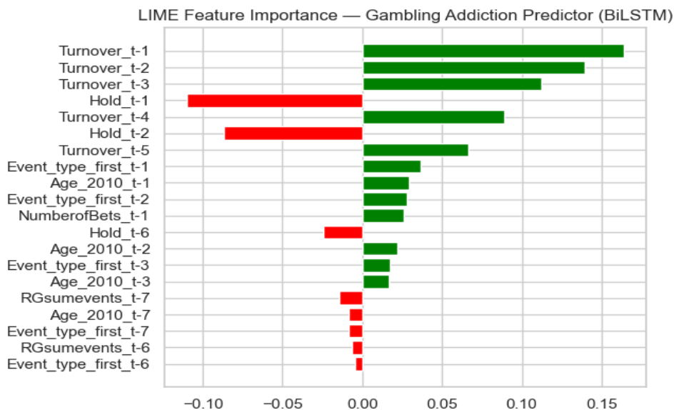
Figure 10: LIME Feature Importance — Gambling Addiction Predictor (BiLSTM)
