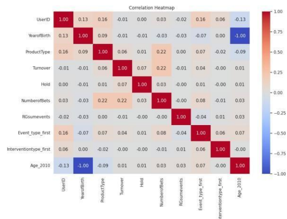
Figure 5: Correlation Heatmap
