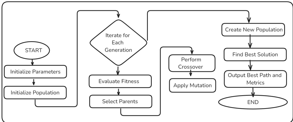
Figure 5: GA Flowchart
