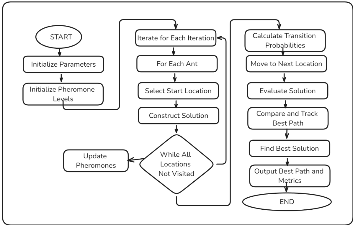
Figure 4: ACO Flowchart
