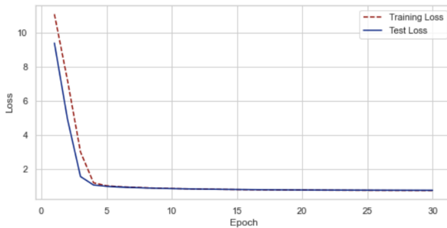
Figure 4: Loss curve for the movie rating prediction
