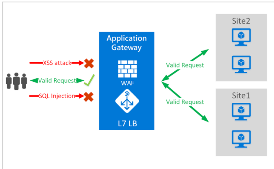
Figure 3: Application Gateway
