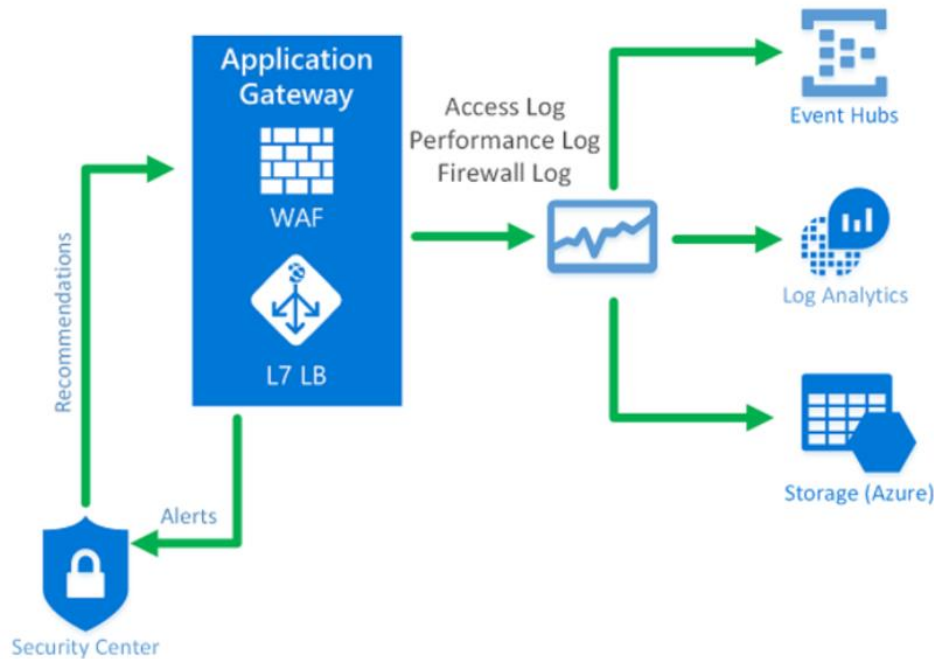
Figure 5: WAF monitoring
