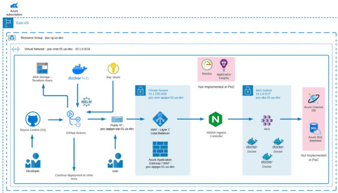
Figure 4:WAF services
