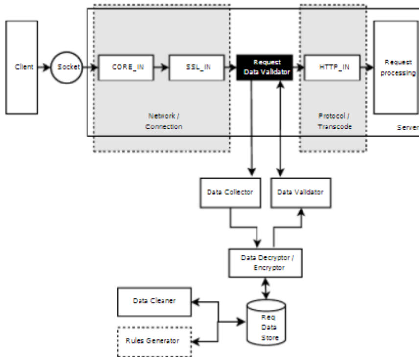
Figure 6: WAF components
