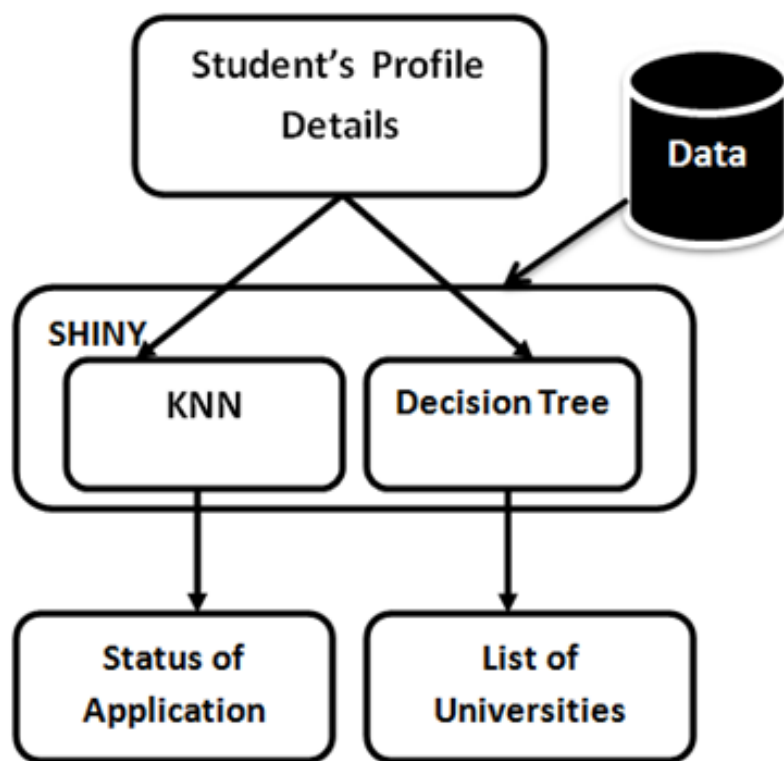
Figure 4: SAP Architecture
