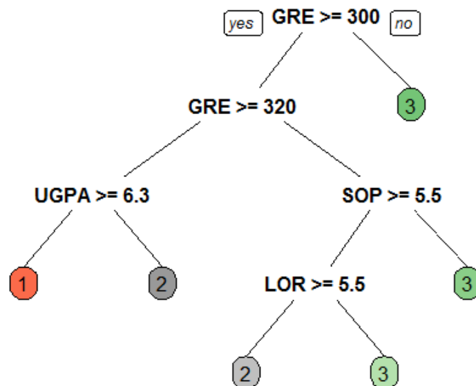
Figure 7: Decision Tree
